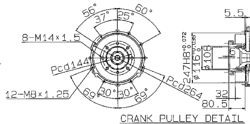
CRANK PULLEY DETAIL
