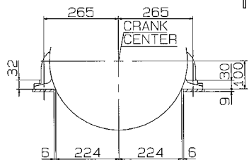
VIEW B
