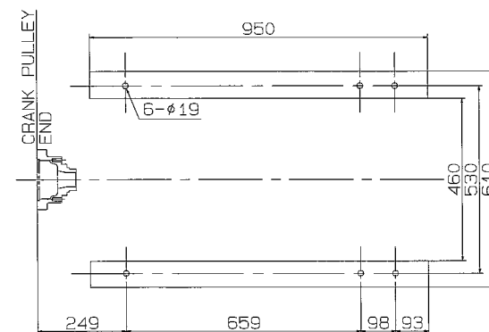
ENGINE MOUNTING
