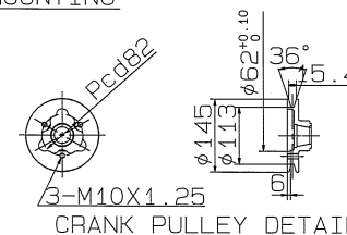
CRANK PULLEY DETAIL
