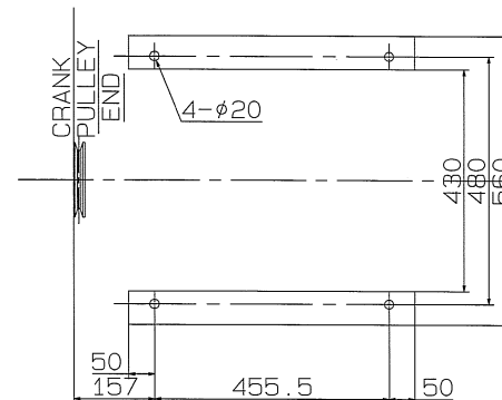
ENGINE MOUNTING
