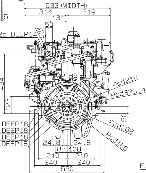
VIEW B
