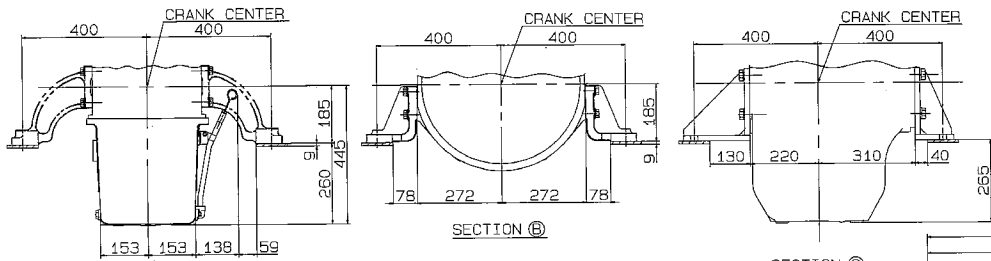
SECTION C
