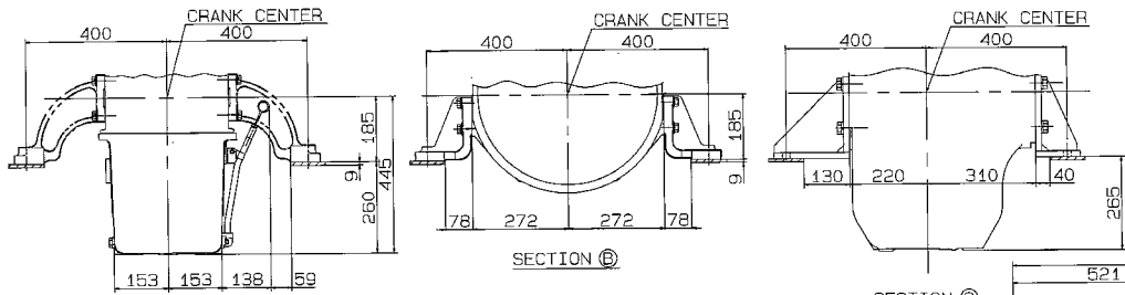
SECTION C
