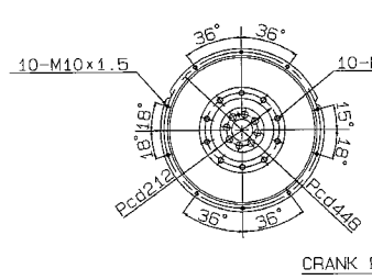
CRANK PULLEY
