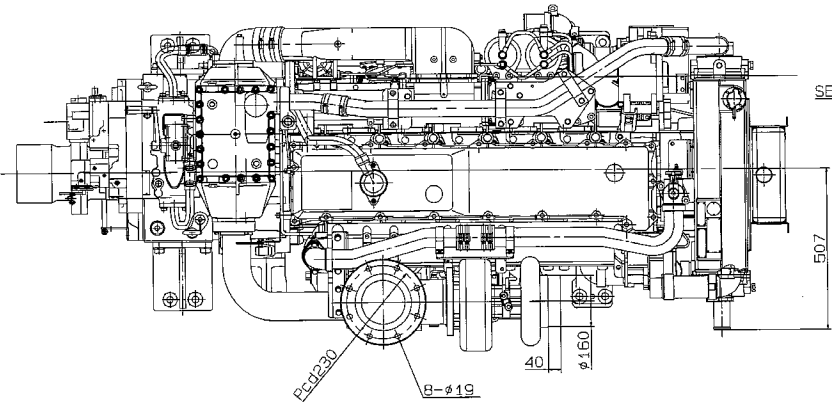
SECTION A
