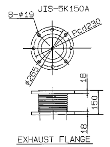
EXHAUST FLANGE
